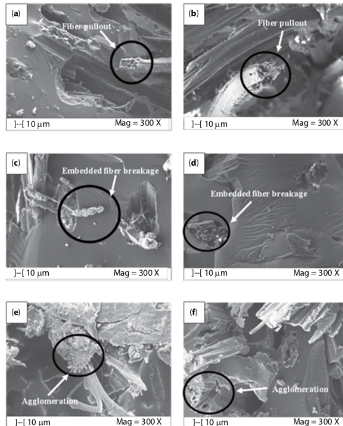
Figure 5 SEM micrographs (at magnification 300×) of (a) NW0, (b) W0, (c) NW3, (d) W3, (e) NW5, and (f) W5.
