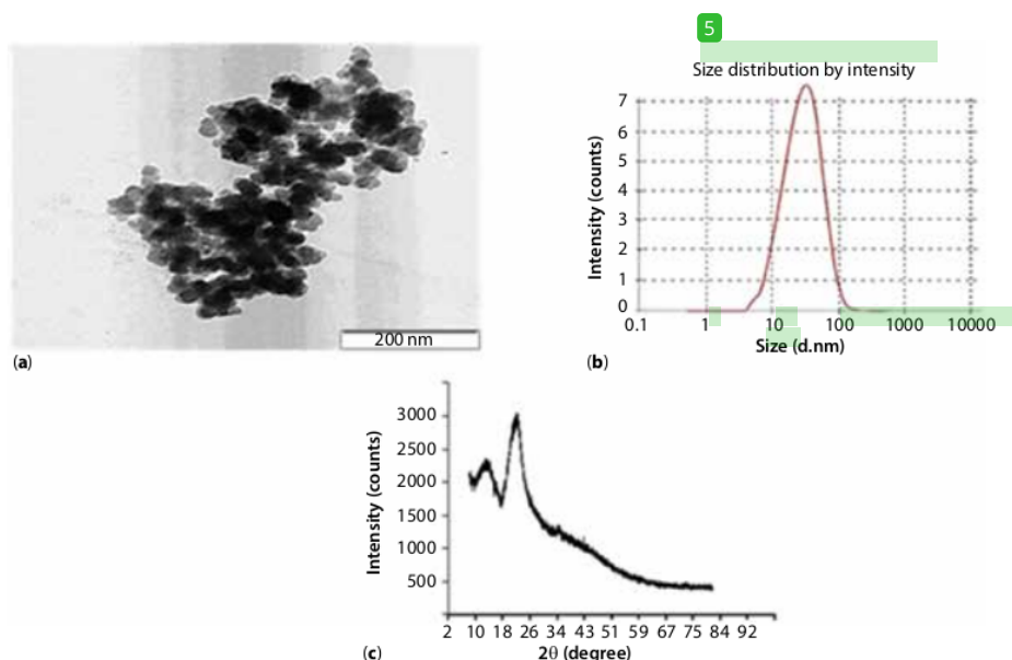
Figure 2 Bamboo nanoparticles: (a) TEM micrograph, (b) size distribution by intensity and (c) X-ray diffractogram.
