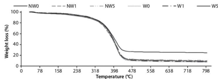
Figure 6 TGA thermograms of reinforced composites with different bamboo nanoparticles filler content.
