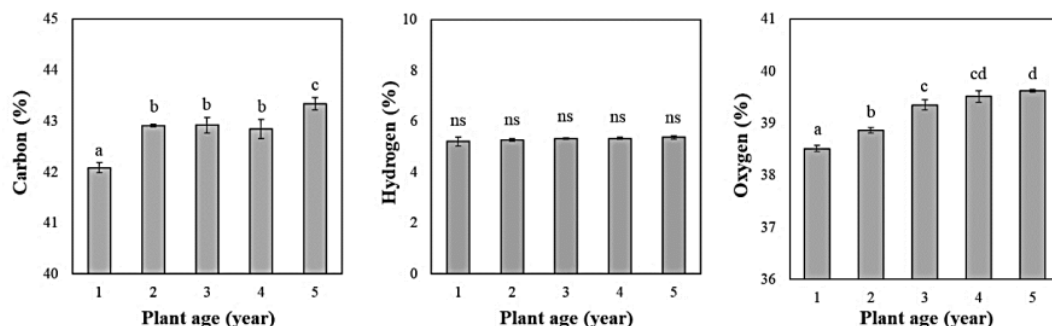
Figure 2. The ultimate composition of Eucalyptus pellita wood at different plant ages. Different letters showed a significant different value at p < 0.05 ; ns = not significant
