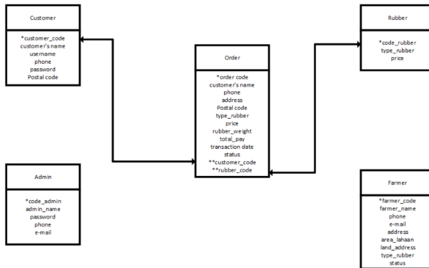
1 Fig.5. Normal form normalization design (2NF=3NF).
