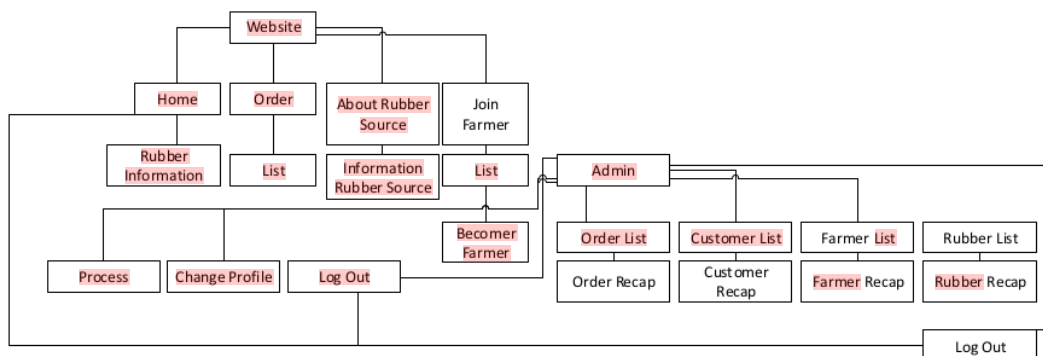
Fig.1. System navigation structure design
