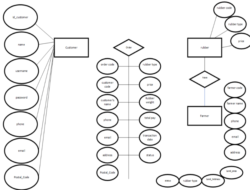
Fig.4. The design of the entity relationship diagram.
