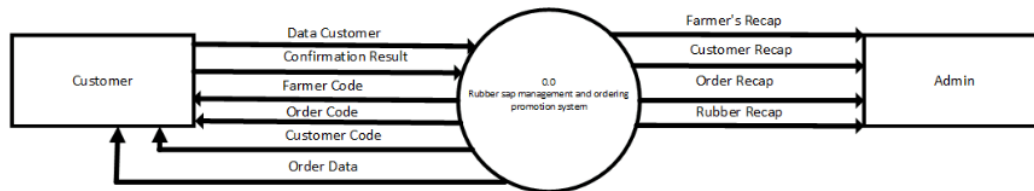
Fig.2. Context diagram design.
