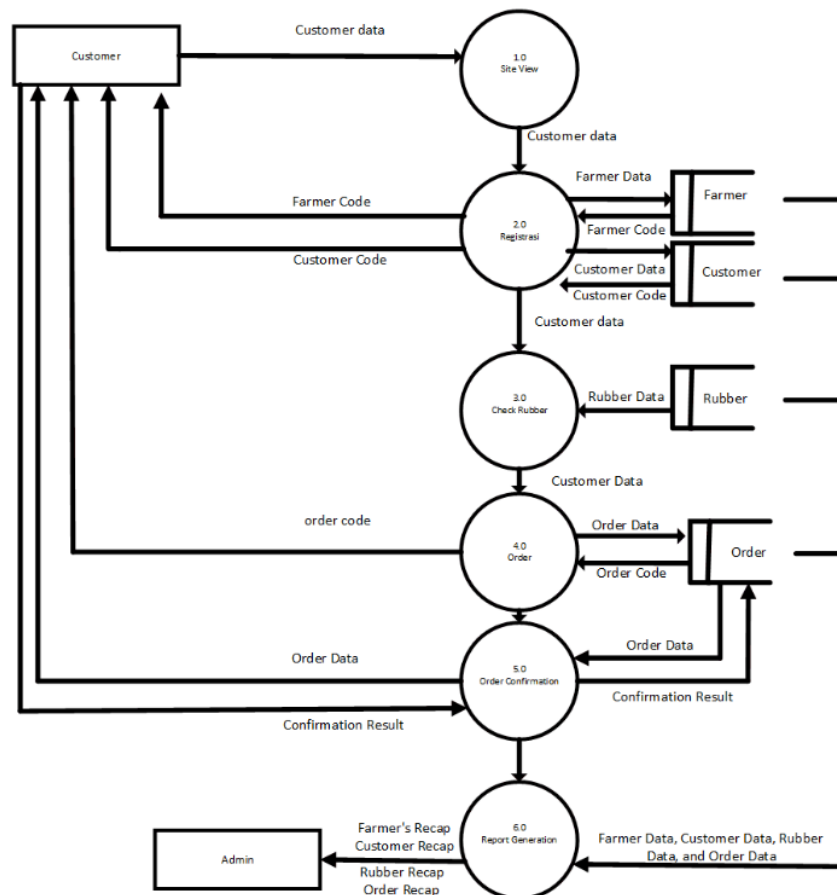
Fig.3. Level 1 diagram design
