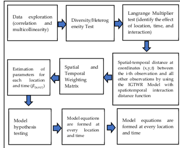
Figure 1. Improved GTWR Model Flowchart.
