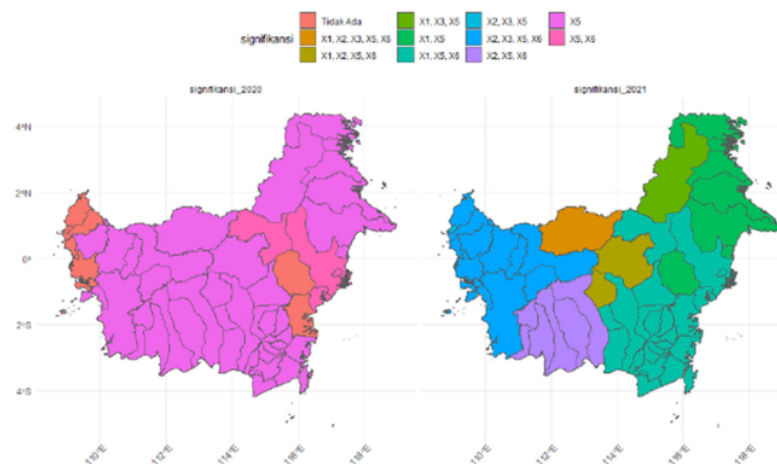
Figure 5. Significance of variables at 5% significance level.
