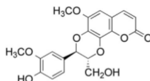
Fig. 2. Structure of cleomiscosin A.
