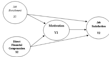
Figure 1. Hypothesis Model
