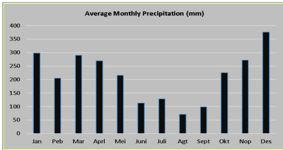
Fig. 3. Average monthly precipitation.
