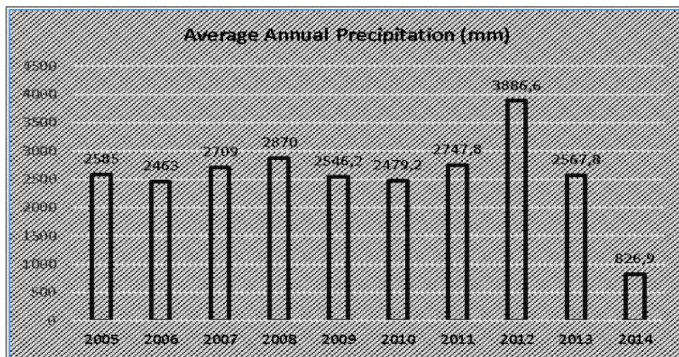
Fig. 2. Average annual precipitation.
