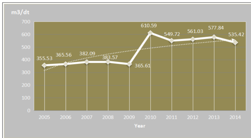
Fig. 4. Average discharge of lately ten years.
