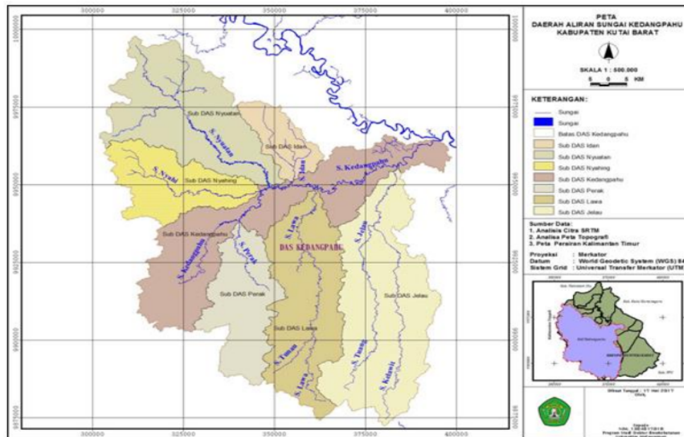
Fig. 1. Location of Kedangpahu Watershed.
