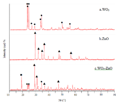
Gambar 1. Hasil XRD (a) \text{WO}_3 , (b) ZnO dan (c) \text{WO}_3\text{-ZnO}
