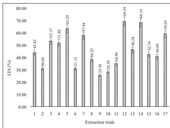
Figure 3. Lipoxygenase inhibitory activity of each extract.
