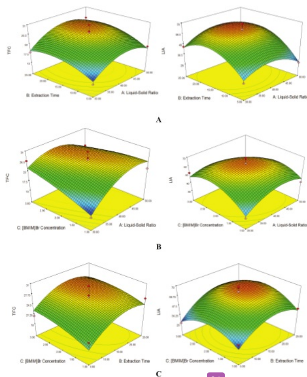
Figure 4. Three dimensional surface and contour plot. (A) Interaction of liquid-solid ratio and extraction time. (B) Interaction of liquid-solid ratio and [BMIM]Br concentration. (C) Interaction of extraction time and [BMIM]Br concentration.
