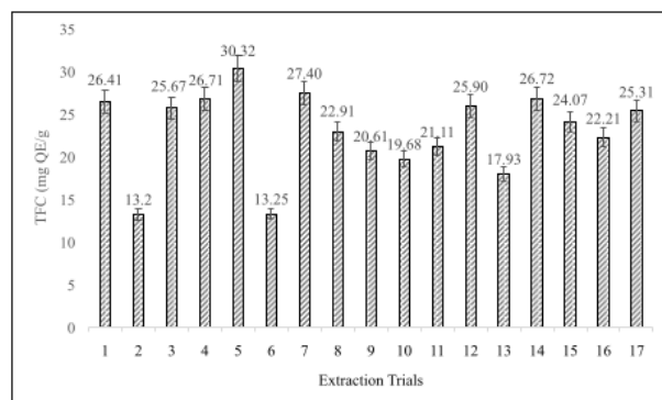
Figure 1. TFC of each extract using IL-MAE method.
