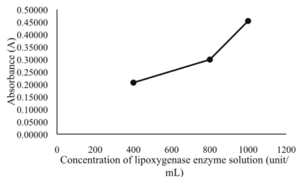
Figure 2. The optimum conditions of lipoxigenase activity inhibition assay. (A) The pH buffer of the boric acid solution, (B) the linoleic acid substrate, and (C) the lipoxigenase enzyme.
