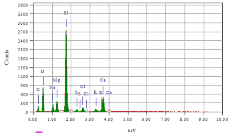
Figure 3. Energy dispersive spectrum of test samples.
