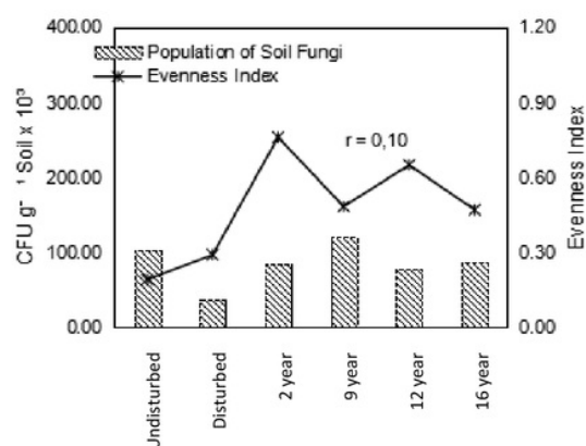
Figure 7. Relationship between index of plants diversity with abundance of soil fungi on post-coal mining reclamation
