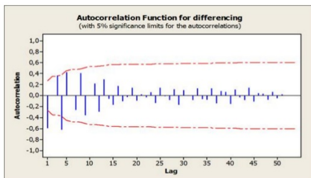
Figure 3 Graph of ACF data on dengue incidence of cases
