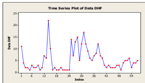
Figure 1 Time series plot data
