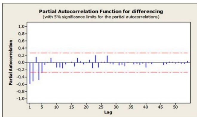
Figure 4 PACF graph of data on seasonal dengue cases is 1, and seasonal differencing order (D) is 0, D = 0 because there was no differencing process for seasonal
