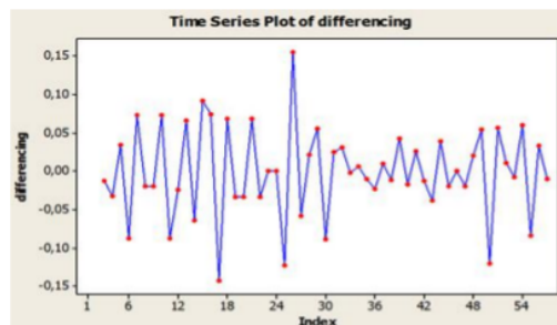
Figure 2 Graph of data after being stationary in averages and variances
