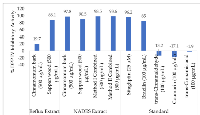
Figure 3. Dipetidyl peptidase IV (DPP IV) Inhibitory Activity of extracts and standards.
