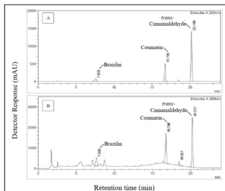
Figure 2. Chromatogram shows (A) a 100 µg/mL mixture of brazilin, coumarin, and trans -cinnamaldehyde standard, and (B) an NADES extract combination of Cinnamomum bark and sappan wood.
