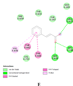
Figure 4. Ligand-Receptor Interaction: (A) Sitagliptin; (B) Braziliin; (C) Coumarin; (D) trans -cinnamaldehyde; and (E) trans -cinnamic acid.
