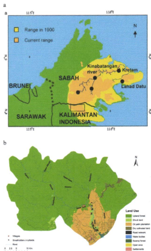
Figure 1 Natural range of Bornean elephant (Fernando et al. 2003) (a) Map of Tulin Onsoi Sub-district, North Kalimantan Province, as part of Bornean elephant ranges with existing land-use (b)
