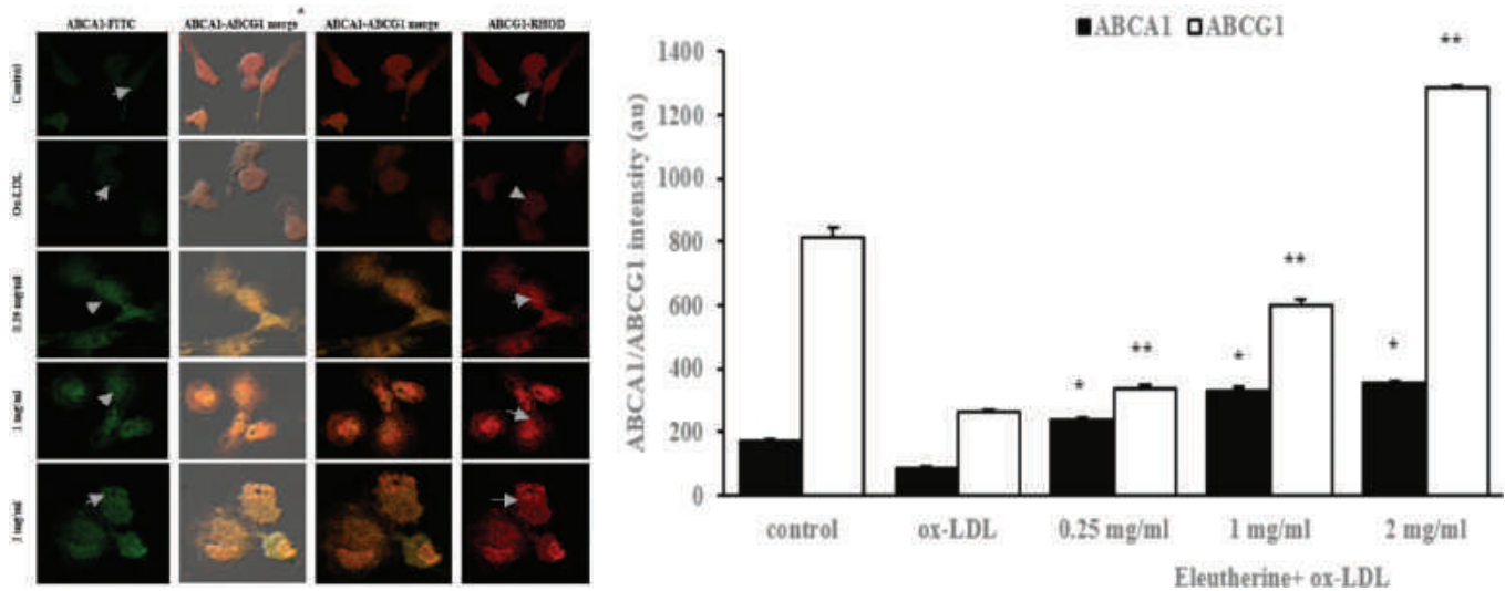
Figure 3. Administration of n-hexane extract of E. americana was able to increase the ABCA1 and ABCG1 protein expression in human macrophages stimulated with ox-LDL. (a) Macrophages derived from PBMCs were given n-hexane extract of 0.25, 1, and 2 mg/ml dosage, incubated for 24 hours, then stimulated with 100 \mu g/ml ox-LDL. After 48 hours of incubation, cells were fixed with 4% paraformaldehyde and double staining immunofluorescence was performed. In (a), the result observed with a confocal microscope demonstrated different levels of intensity (green color) that showed ABCA1 expression, while the red color showed ABCG1 protein expression. (b) The result of quantitative color intensity measurements in the treatment group was decreased compared to the control group with *p = 0.000 . All data are presented as mean \pm SEM.
