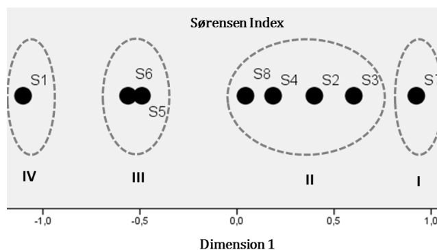
Figure 2. The group classification and close relationship of butterfly habitats based on Sørensen index calculations
