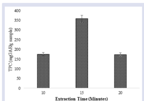
Figure 4: The optimum single factor of extraction time on polyphenols extraction from M. speciosa .
