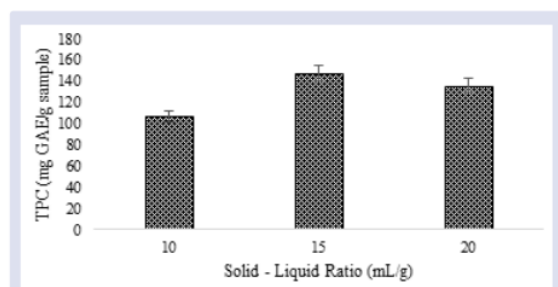
Figure 2: The optimum single factor condition of solid-liquid ratio on polyphenol extraction from M. speciosa leaves.
