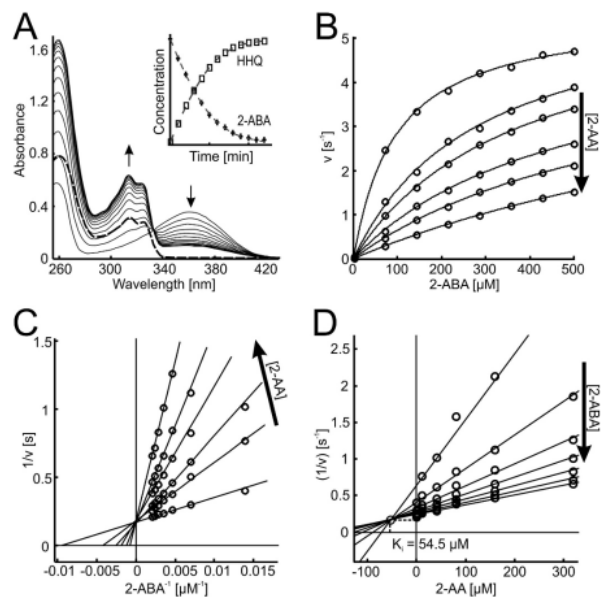
FIGURE 7. Steady-state kinetics and competitive inhibition of PqsBC by 2-AA. A, conversion of 2-ABA ( \lambda_{max} at 360 nm) and octanoyl-CoA (absorbing at 260 nm) to HHQ ( \lambda_{max} at 313 nm). 20 nM PqsBC was mixed with 50 \mu M of each substrate. Spectra were measured every 25 s with a bandwidth of 1 nm. HHQ formation could be observed at 313 nm with a differential extinction coefficient of 6,520 M^{-1} cm^{-1} . The remaining absorption above 340 nm after full conversion of the substrates (bold trace) is due to scattering and can be eliminated by diluting to 50% in 2-propanol/HCl (dashed trace). Inset, conversion of 10 \mu M substrates, monitored at 313 nm (HHQ) and 360 nm (2-ABA) with the determined extinction coefficients. Data interval is 1 min. B–D, inhibition of PqsBC activity by 2-AA. B, nonlinear fits of measured initial rates. The Lineweaver-Burkplot (C) shows the characteristic pattern of competitive inhibition. Using the Dixon plot (D), the inhibitor constant K_i of the competitive reaction could be determined graphically. Experiments were performed with 50 \mu M octanoyl-CoA and 20 nM PqsBC in HEPES buffer, pH 8.2, at 25 °C; arrows indicate ascending concentrations.
