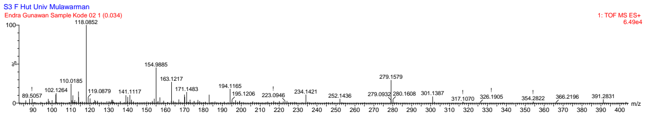
Figure 2 LCMS analysis results of O. palindan fruit extracted with hot water.
