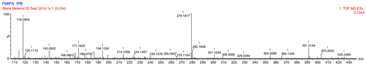
Figure 1 LCMS analysis results of O. palindan fruit extracted with room temperature water.
