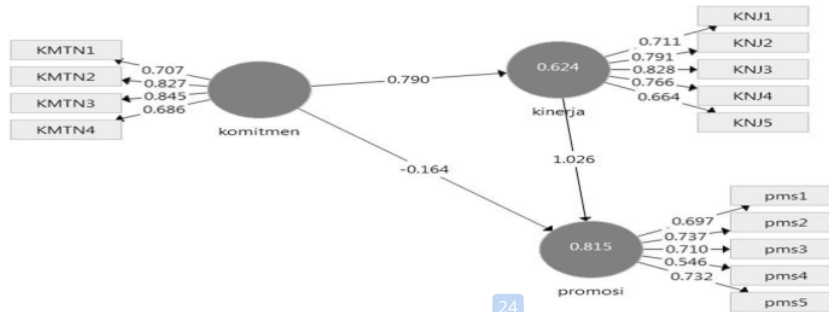
Gambar 1. Hasil outer loading (convergent validity)
