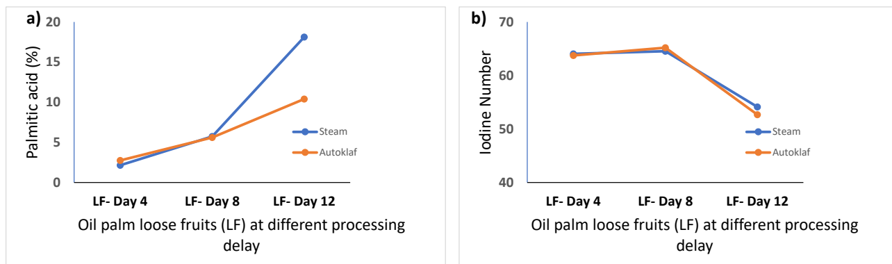
Figure 6. The effect of processing delay on a) Palmitate acid content and b) Iodine number in steaming and autoclaving processes.
