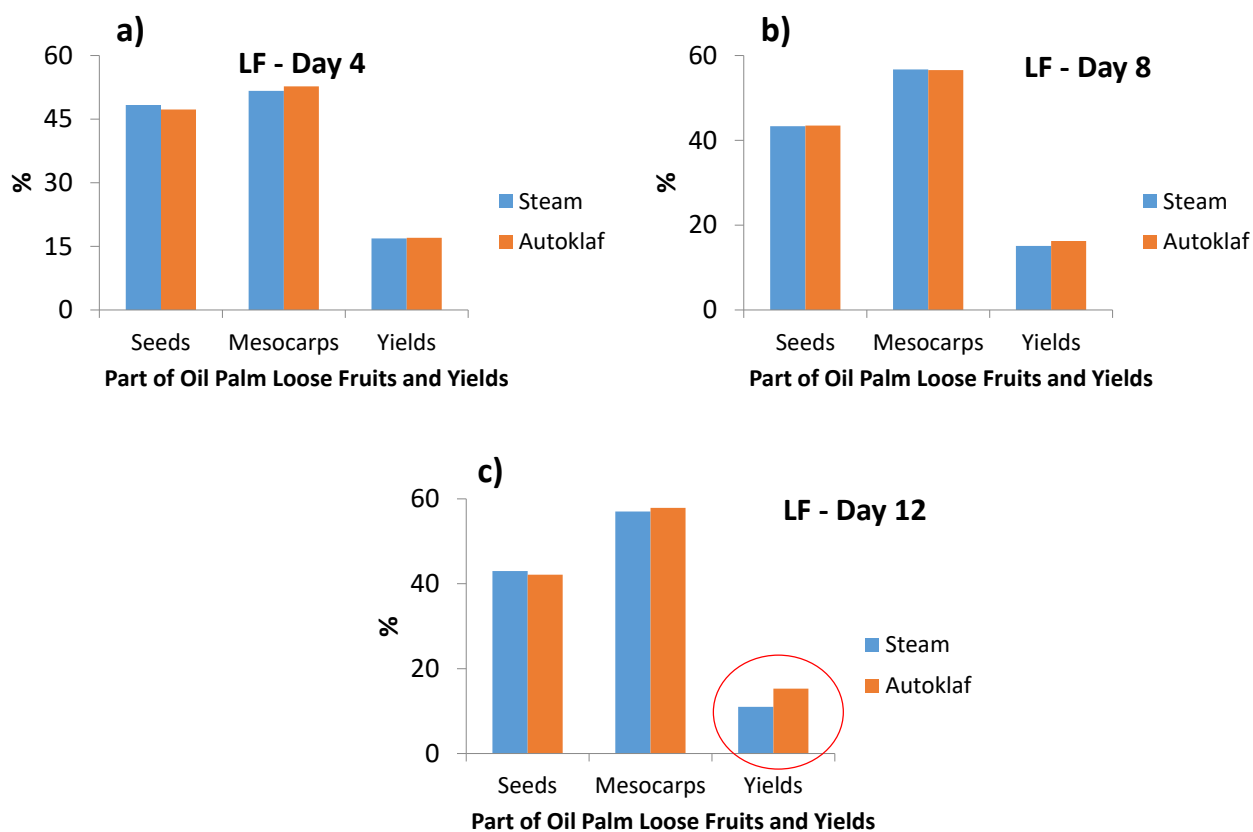
Figure 3. Percentage of seeds, mesocarps and yields of oil palm loose fruits (LF) at different processing delay.
