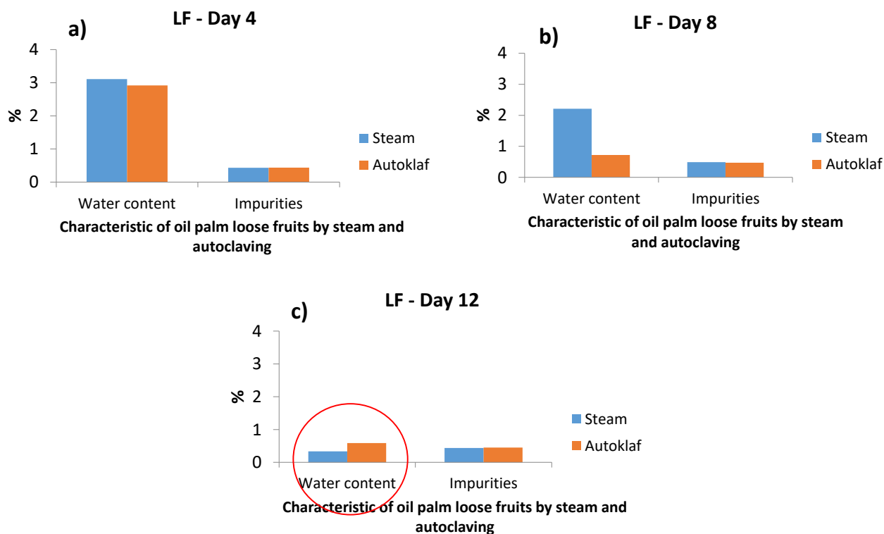
Figure 4. Water content and impurities of oil palm loose fruits (LF) at different processing delay.
