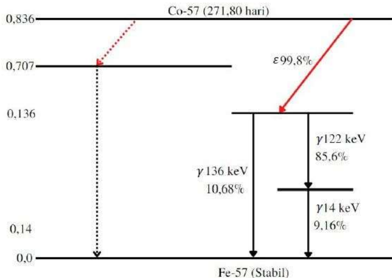
Gambar 3. Peluruhan Cobalt-57 (Co-57) (IAEA, 2007).
