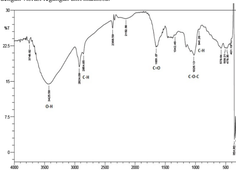
Gambar 1. Spektra FT-IR Glukomanan Umbi Porang ( Amorphophallus muelleri )
