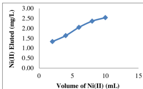
Figure 5. Effect of Ni(II) ions volume
