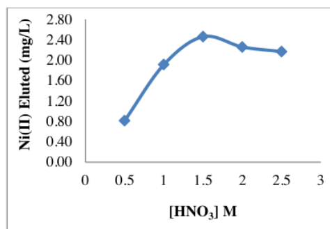
Figure 3. Effect of \text{HNO}_3 concentration as eluent
