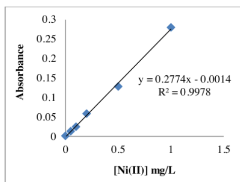
Figure 6. Calibration curve of Ni(II) standard.
