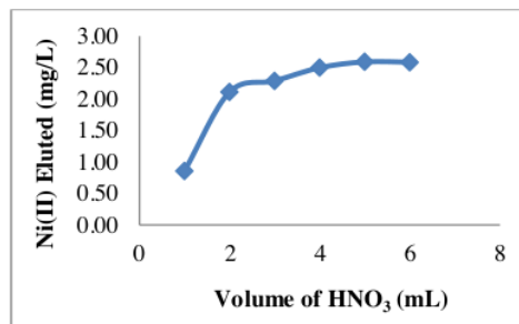
Figure 4. Effect of volume \text{HNO}_3 as eluent
