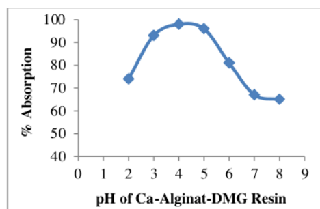
Figure 1. Effect of pH of Ca-alginate-DMG resin in the absorption of Ni (II).
