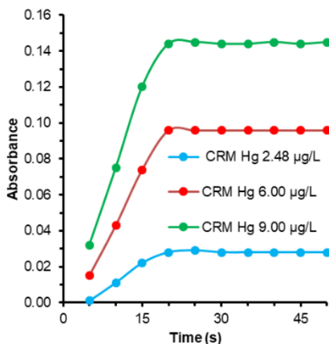
Fig 1. Reading delay time variation chart
