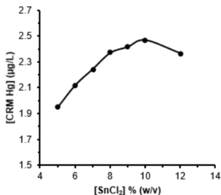
Fig 2. Influence of SnCl 2 concentration
