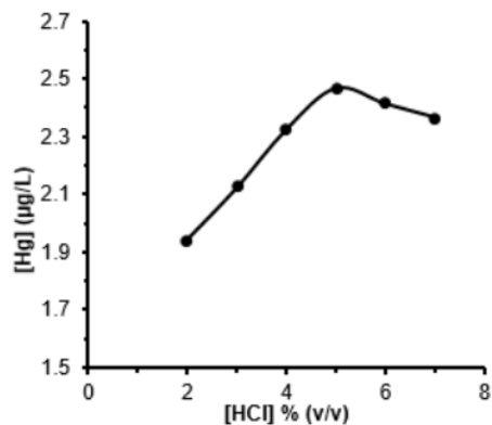
Fig 3. Influence of HCl concentration
