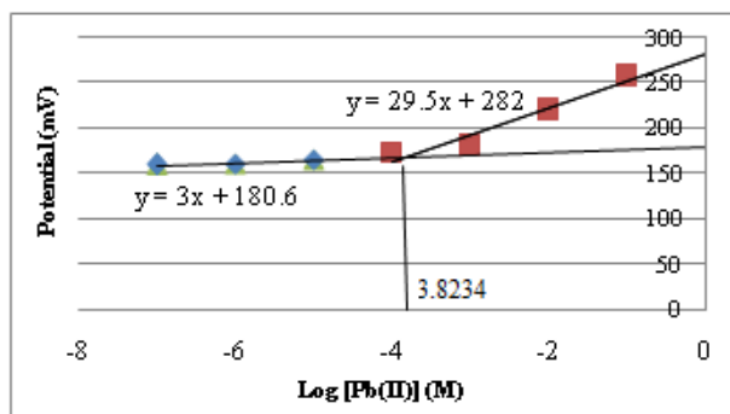
Fig. 3. Determination of Nernstian Slope and Detection Limit
