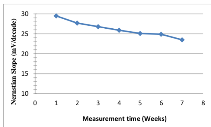
Fig. 6. Nernstian Slope Measurement for every week
