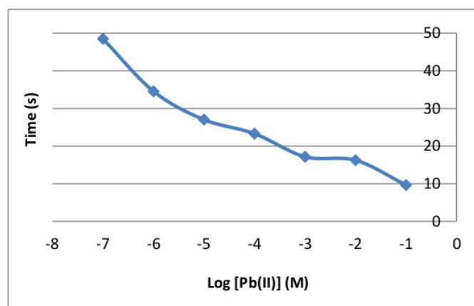
Fig. 5. Effect of Concentration Against Response Time
