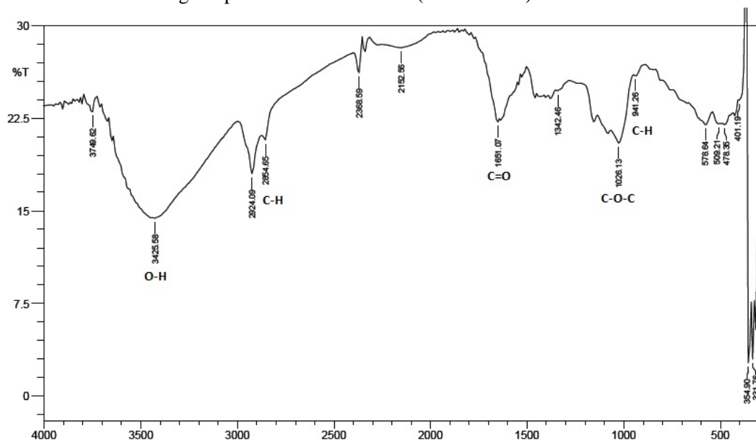
Gambar 1. Spektra FT-IR Glukomanan Umbi Porang ( Amorphophallus muelleri )
