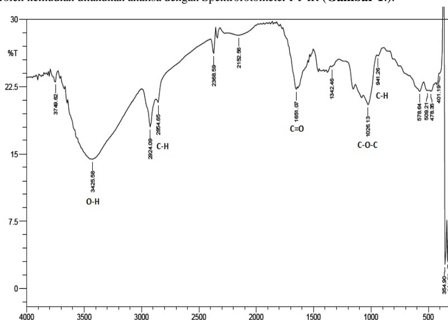
Gambar 1. Spektra FT-IR Glukomanan Umbi Porang ( Amorphophallus muelleri )
