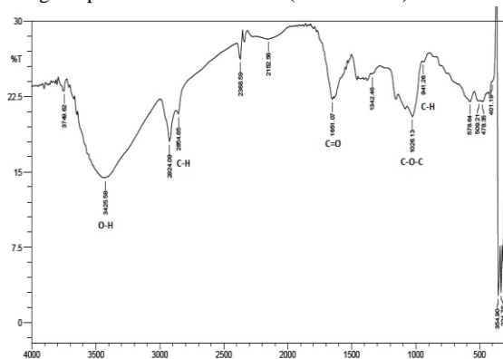
Gambar 1. Spektra FT-IR Glukomanan Umbi Porang ( Amorphophallus muelleri )
