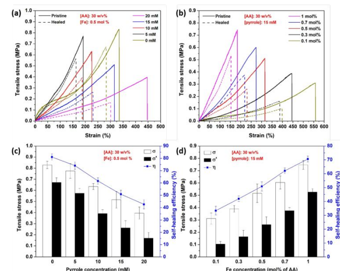
Figure 5. Mechanical properties of tensile stress-strain curves of hydrogels with (a) variation of pyrrole concentration; and (b) variation of Fe concentration. Tensile stress-self-healing efficiency graphs of hydrogels with (c) variation of pyrrole concentration; and (d) variation of Fe concentration.
