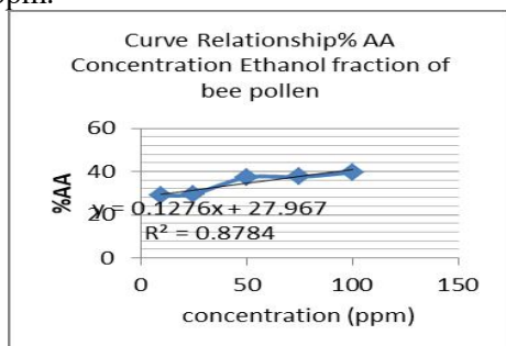
Figure 1. Graph of IC 50 values on the ethanol fraction of bee pollen
