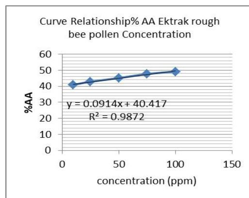
Figure 4. Graph of IC 50 values on the extract crude of bee pollen
