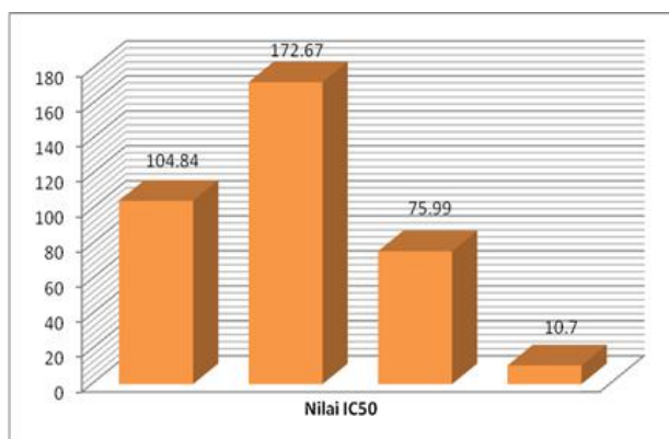
Figure 5. Graph of IC 50 Values on the Graph image extract crude, the fraction of ethanol and ethyl acetate fraction, and vitamin C
