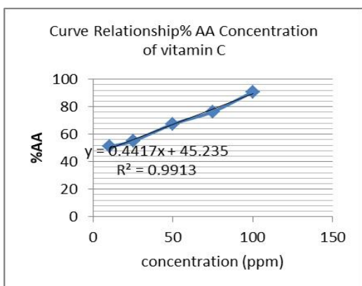
Figure 3. Graph of IC 50 Values on the concentration vitamin C of bee pollen
