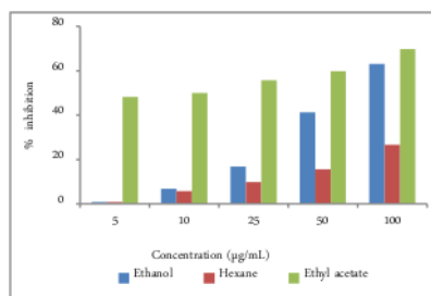
Figure 1. Antioxidant potential from different crude extract from E. balikpapanensis against DPPH
