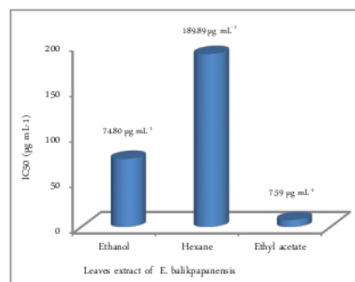
Figure 2. IC_{50} value from ethanol, hexane, and ethyl acetate leaves extract of E. balikpapanensis
