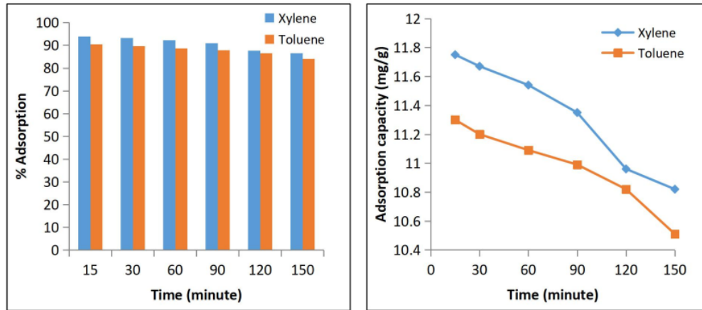
Figure 6. % Adsorption and Adsorption Capacity (SBA-15 mass = 0.1 grams, concentration of toluene and xylene = 25 mg/L)
