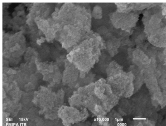
Figure 4. SEM picture of SBA-15 material from rice husk ash
