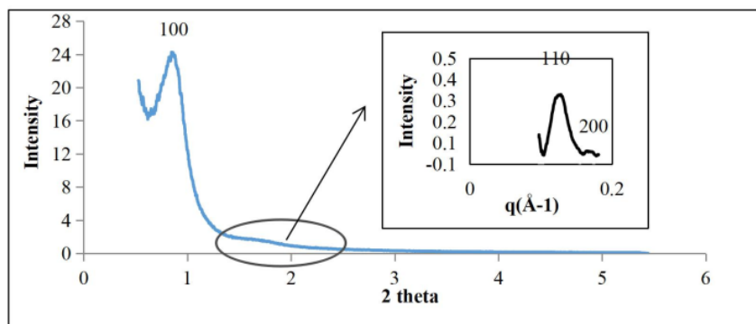
Figure 2. SAXS Pattern of SBA-15 Rice Husk Ash
