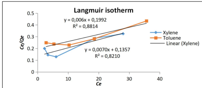
Figure 7. Langmuir Isotherm Graph
