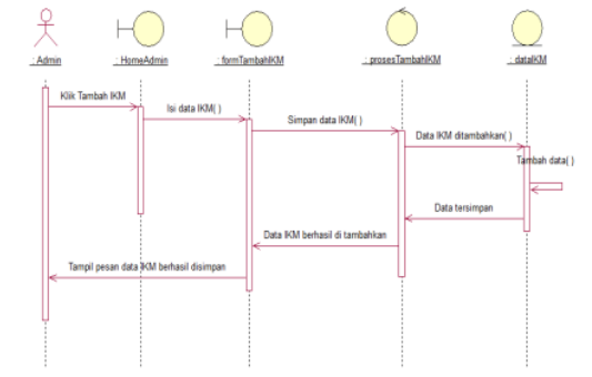
Gambar. 6. Sequence Diagram Tambah Data IKM
