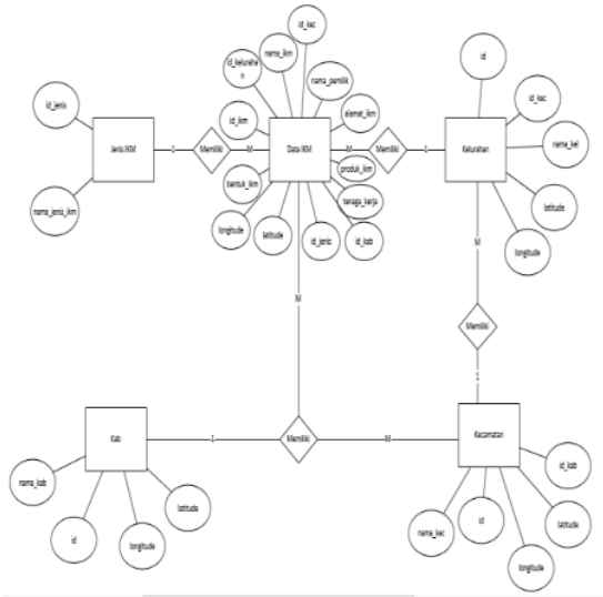
Gambar. 7. Entity Relationship Diagram
