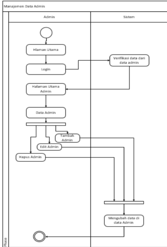
Gambar. 4. Activity Diagram Manajemen Admin
