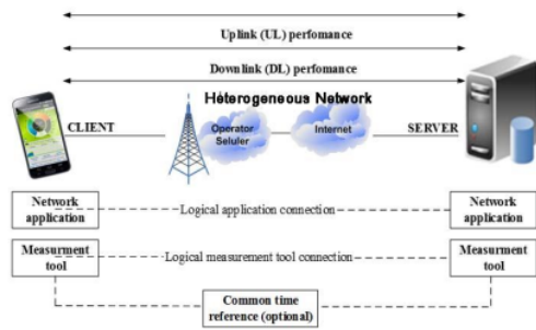
1 Figure 2: Measurement architecture
