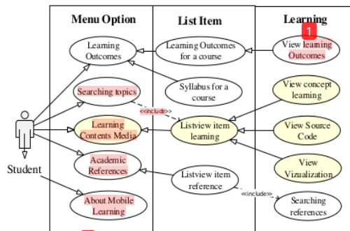
Figure 3: Use case diagram for students
