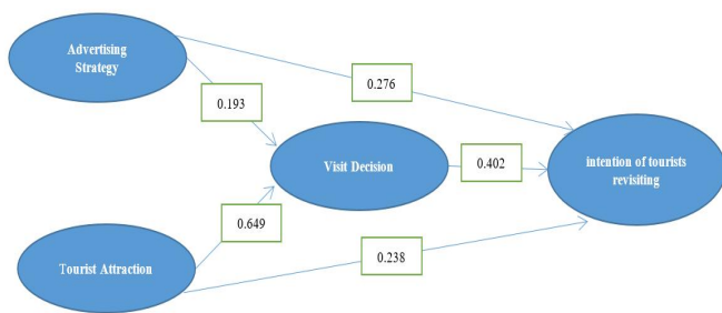
Figure 1. Path analysis chart
