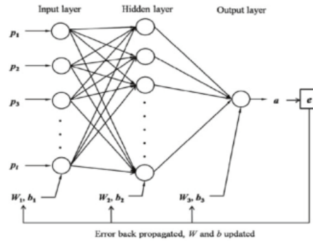
Fig. 1. A typical structure of BPNN architecture [17]
