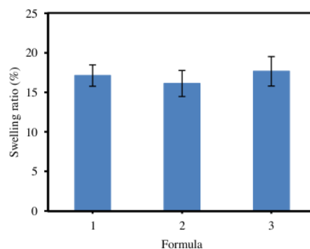
Fig. 4: Swelling ratio of F1 to F3 formulations
