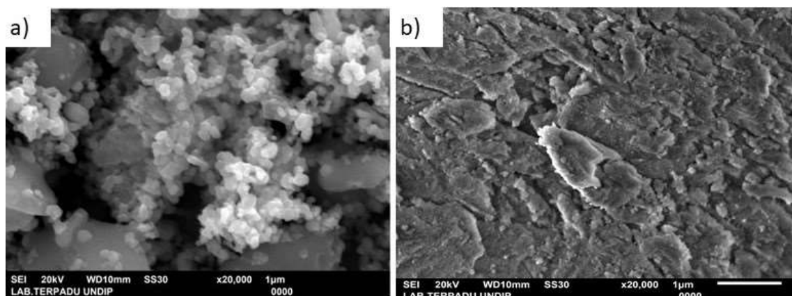
Figure 2. Differences in surface morphology of the TiO 2 layer on ITO glass (a) before and (b) after immersion in Mahkota Dewa extract dye with a magnification of 20,000x
