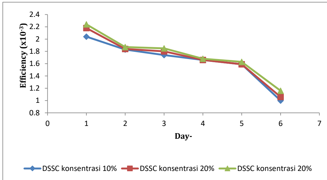
Figure 4. Curve of DSSC efficiency decline with time
