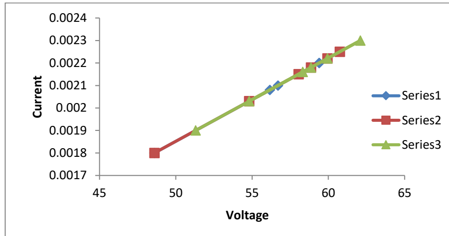
Figure 3. Current and voltage curve of DSSC TiO 2 and dye concentration of 10%
