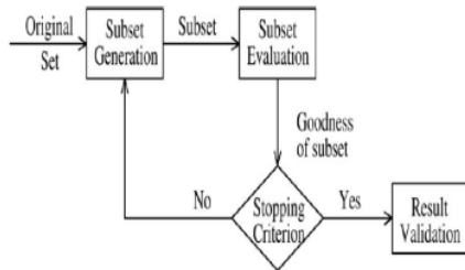
Fig. 2. The Feature Selection System
