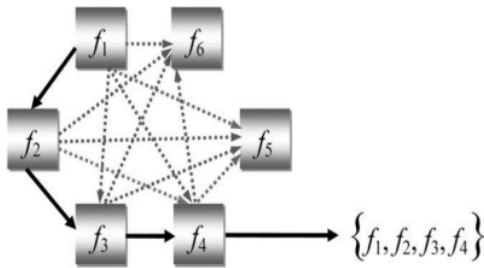
Fig. 4. ACO representation for Feature Selection
