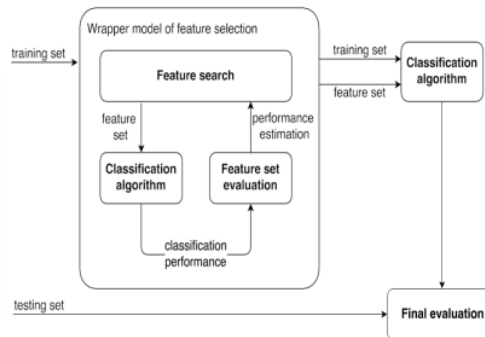
Fig. 3. General structure for wrapper models of feature selection
