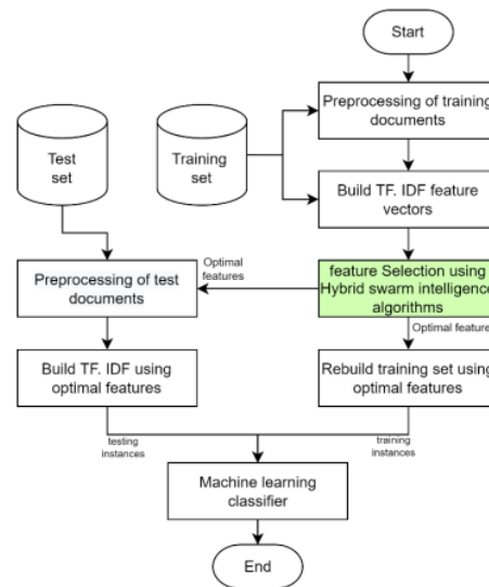
Fig. 6. Block diagram text categorization
