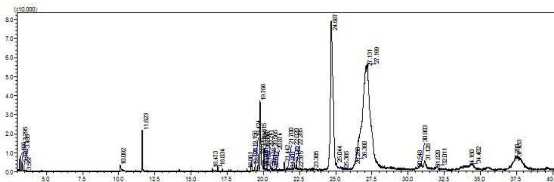
Figure 1. GC chromatogram of ethyl acetate fraction of C. tomentosa (Blume) root
