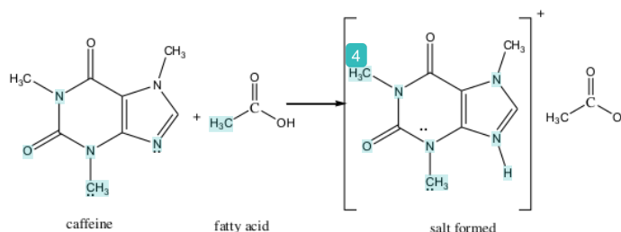
Figure 2. Reaction between caffeine with free fatty acid
