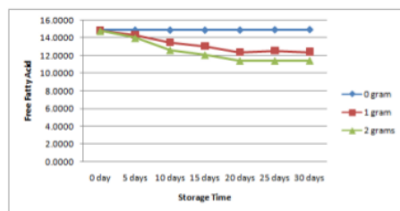
Figure 1. FFA content at various variations a addition of crude extract tea leaves and duration of storage on crude palm oil
