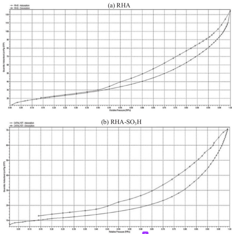
3 FIGURE 3. N 2 adsorption-desorption isotherms of RHA and RHA-SO 3 H
