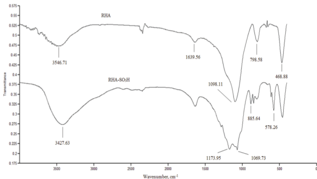
FIGURE 2: FTIR spectra of RHA and RHA-SO 3 H
