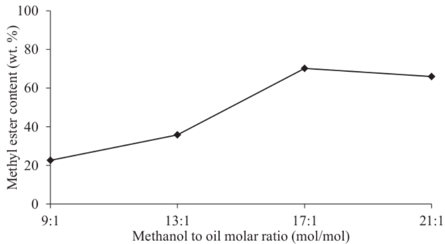
9 FIGURE 8. Effect of methanol to DC-oil molar ratio (reaction conditions: 6 wt.% catalyst at 120 °C for 5 h)
