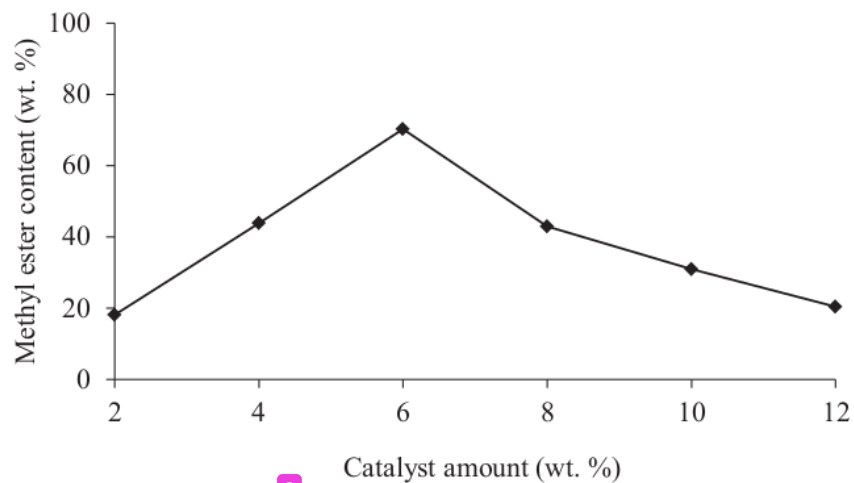
39 2 FIGURE 7. Effect of catalyst amount on methyl ester yield at 120 °C, methanol to oil molar ratio of 17:1 for 5 hours
