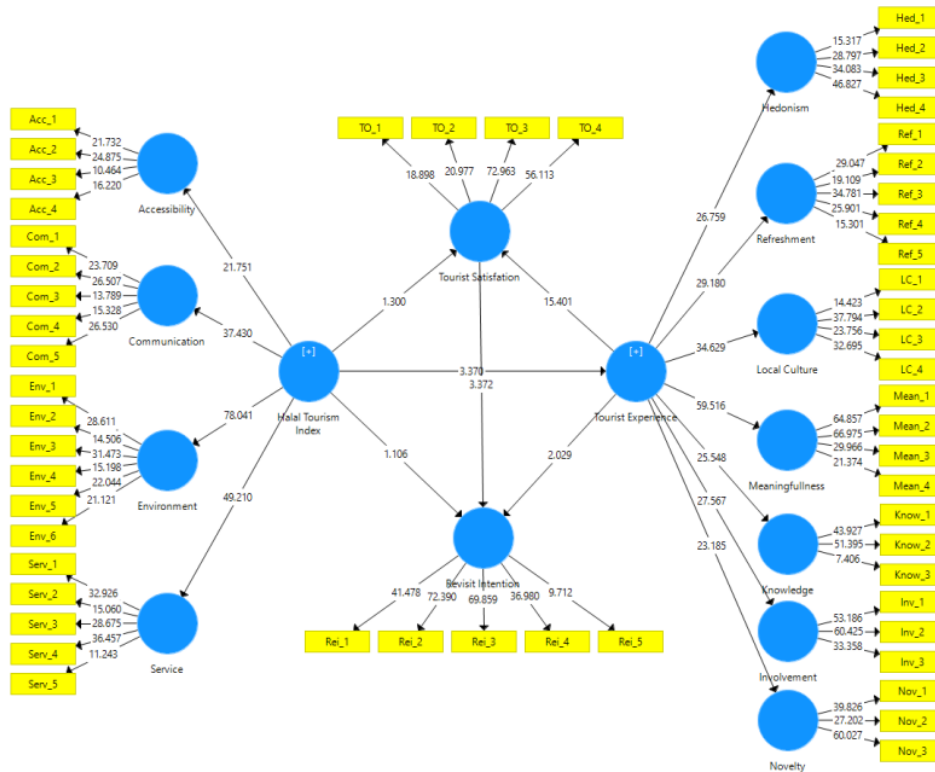
Fig. 2. Bootstrapping construct
