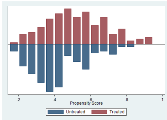
Figure 1. Propensity score distribution and common support.
