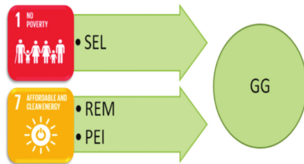
Figure 3: Model report
