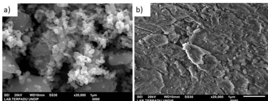
Figure 2. Differences in surface morphology of the TiO 2 layer on ITO glass (a) before and (b) after immersion in Mahkota Dewa extract dye with a magnification of 20,000x.
