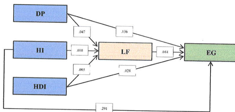
Figure 1: Complete relationship of regression
