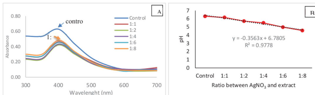
5 FIGURE 2. (A) UV-VIS spectra of silver nanoparticles synthesized using aqueous extract of ant nest plant ( Myrmecodia pendans ) bulb. Control = Myrmecodia pendans bulb crude extract without \text{AgNO}_3 addition. Ratio 1:8 = 0.5 M \text{AgNO}_3 and 10 % of M. pendans bulb crude extracts. (B) The degree acidity of the silver nanoparticles solution system synthesized using different ratio aqueous extract of ant nest plant ( Myrmecodia pendans ) bulb.
