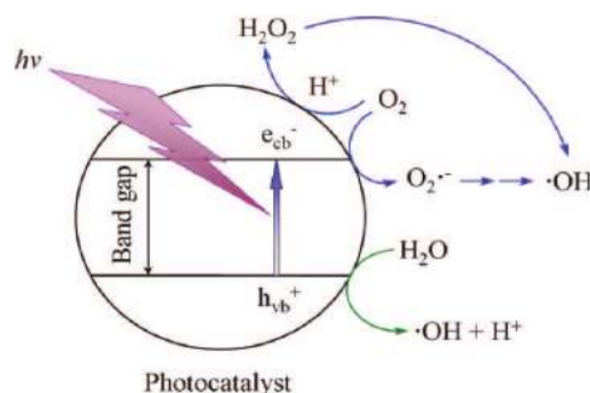
Figure 1. Schematic representation of semiconductor photocatalytic mechanism [8].
