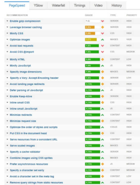
Fig. 3. Recommendation and grade of pagespeed results
