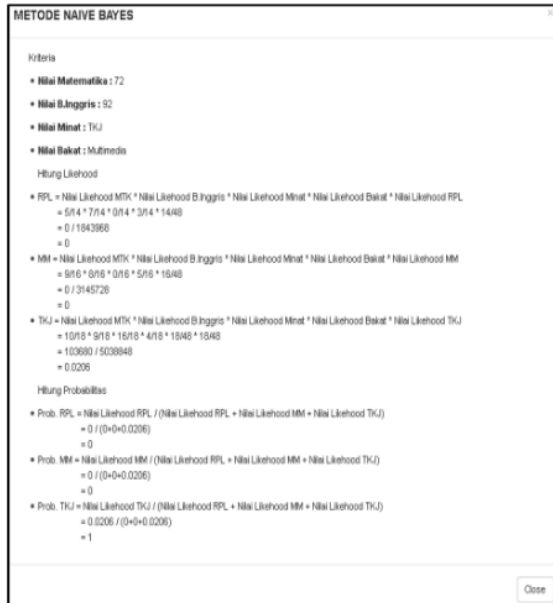
Fig. 3. Calculation Results Naïve Bayes
